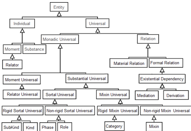
Figure 1. Excerpt of UFO taxonomy[2]
