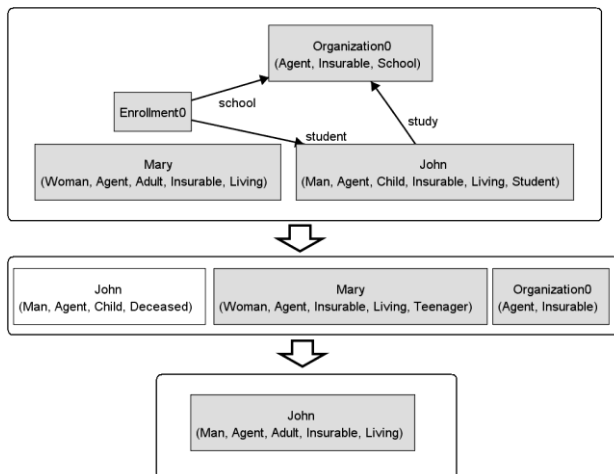
Figure 3. A sequence of states
