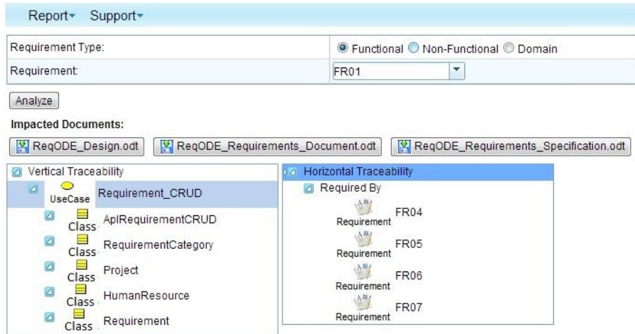
Fig. 2. Supporting Impact Analysis of a Requirement Change
