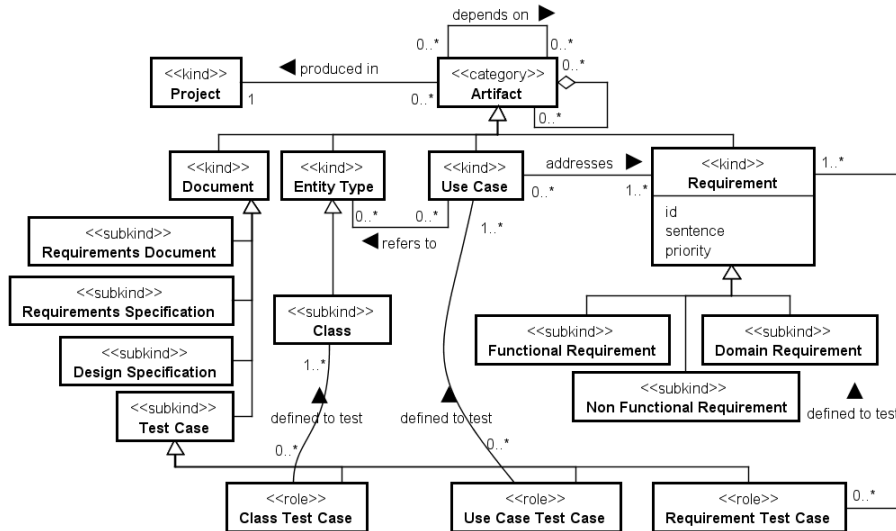
Fig. 1. A fragment of the Software Requirements Ontology
