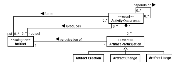
Fig. 4. The “Work Product Participation” (WPPA) pattern.
