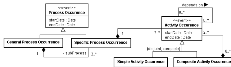
Fig. 2. The “Process and Activity Execution” (PAE) pattern.
