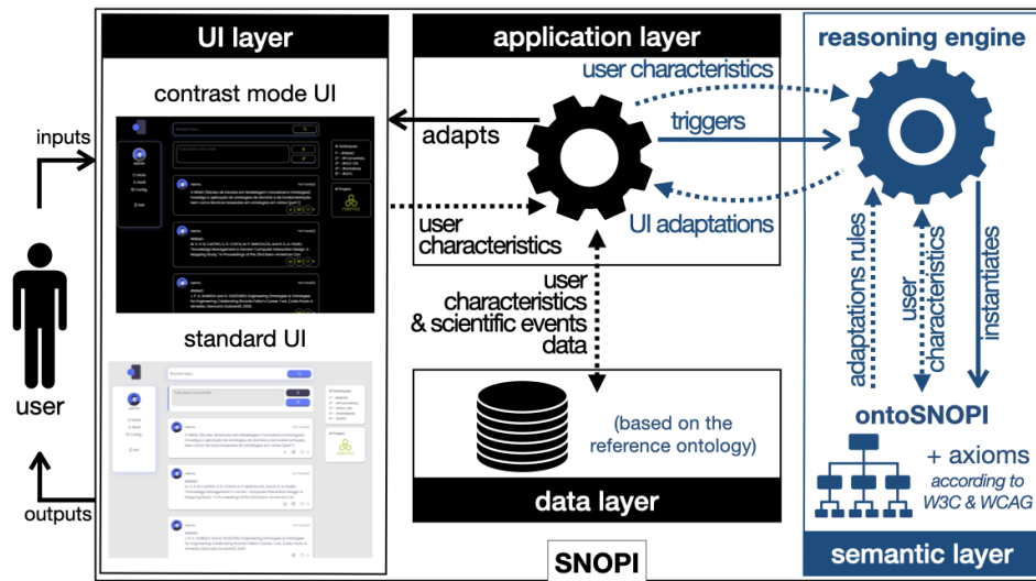
Figure 4: SNOPI architecture overview.
