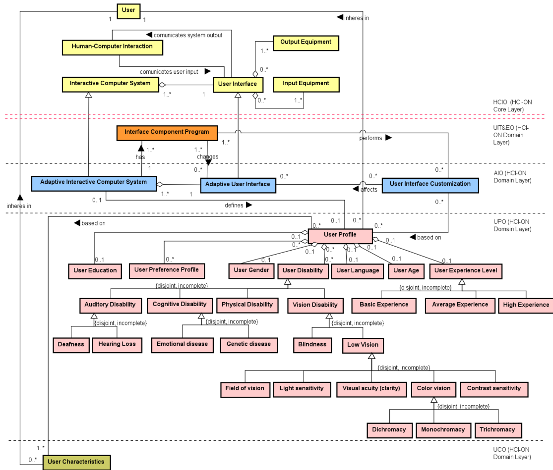
Figure 3: HCI-ON fragment involving AUI system concepts.
